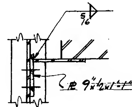
SECTION E-E
