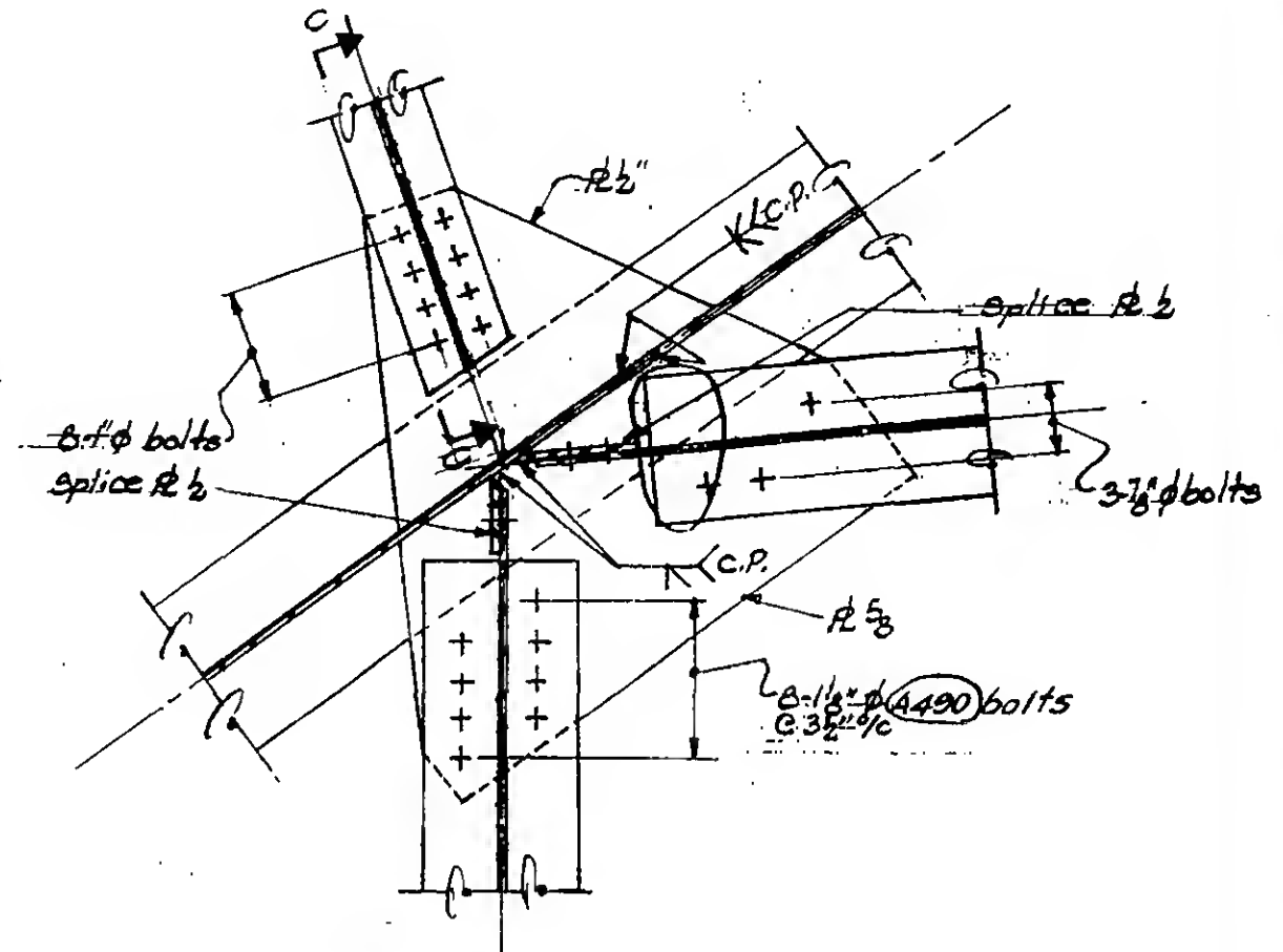
Section b-b
