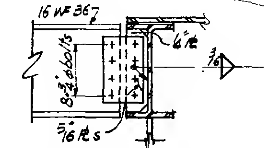
SECTION h-h (DETAIL 810 B ONLY)
