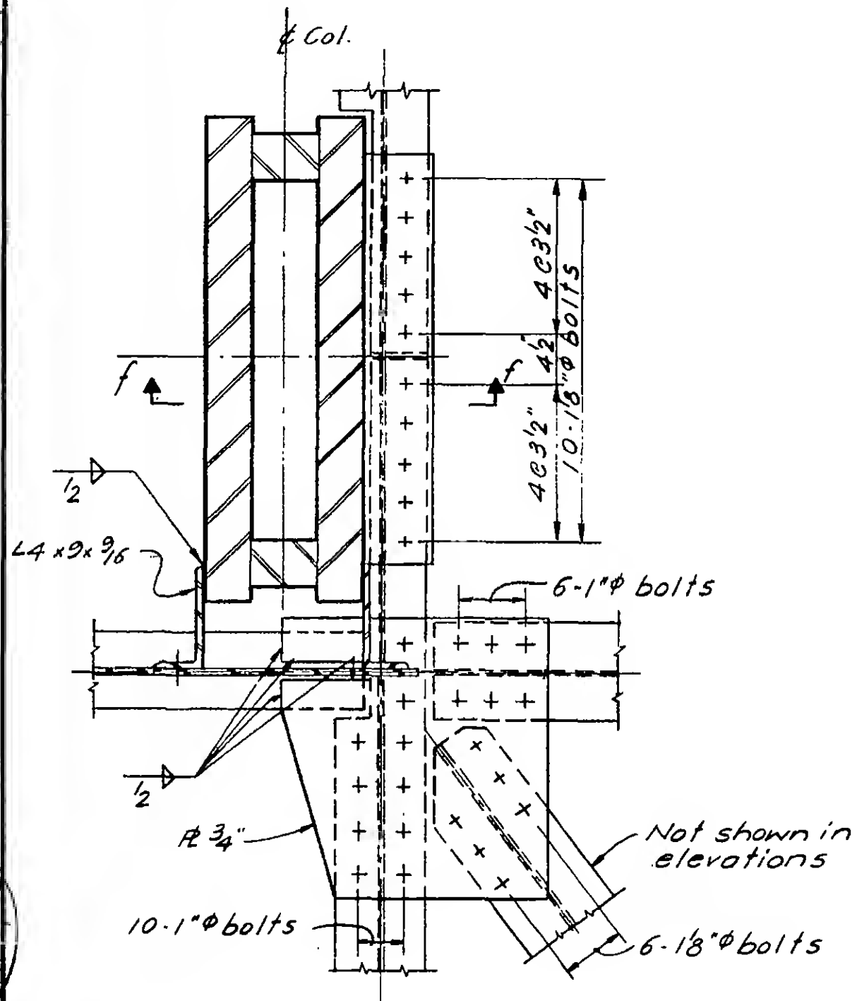
Section c-c
