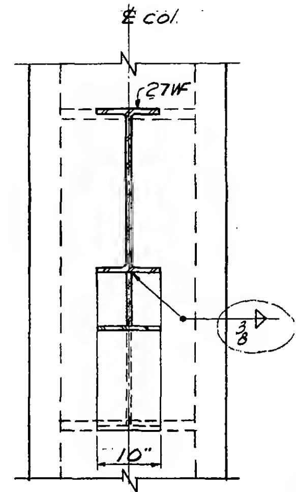
Section b-b
