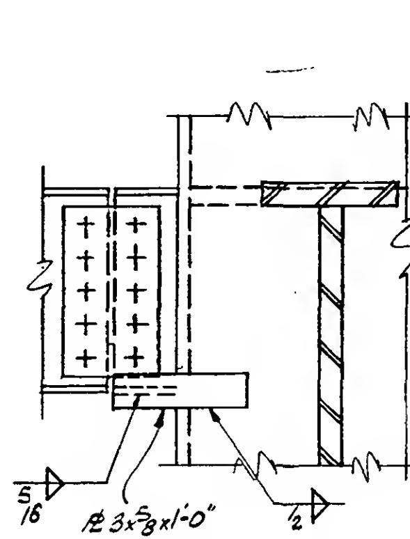
Section c-c, Opp. hand
