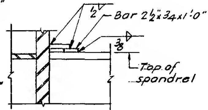
Section e-e
