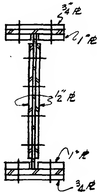
SECTION b-b
