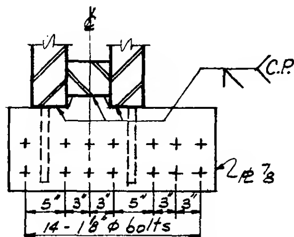
SECTION 6-6
