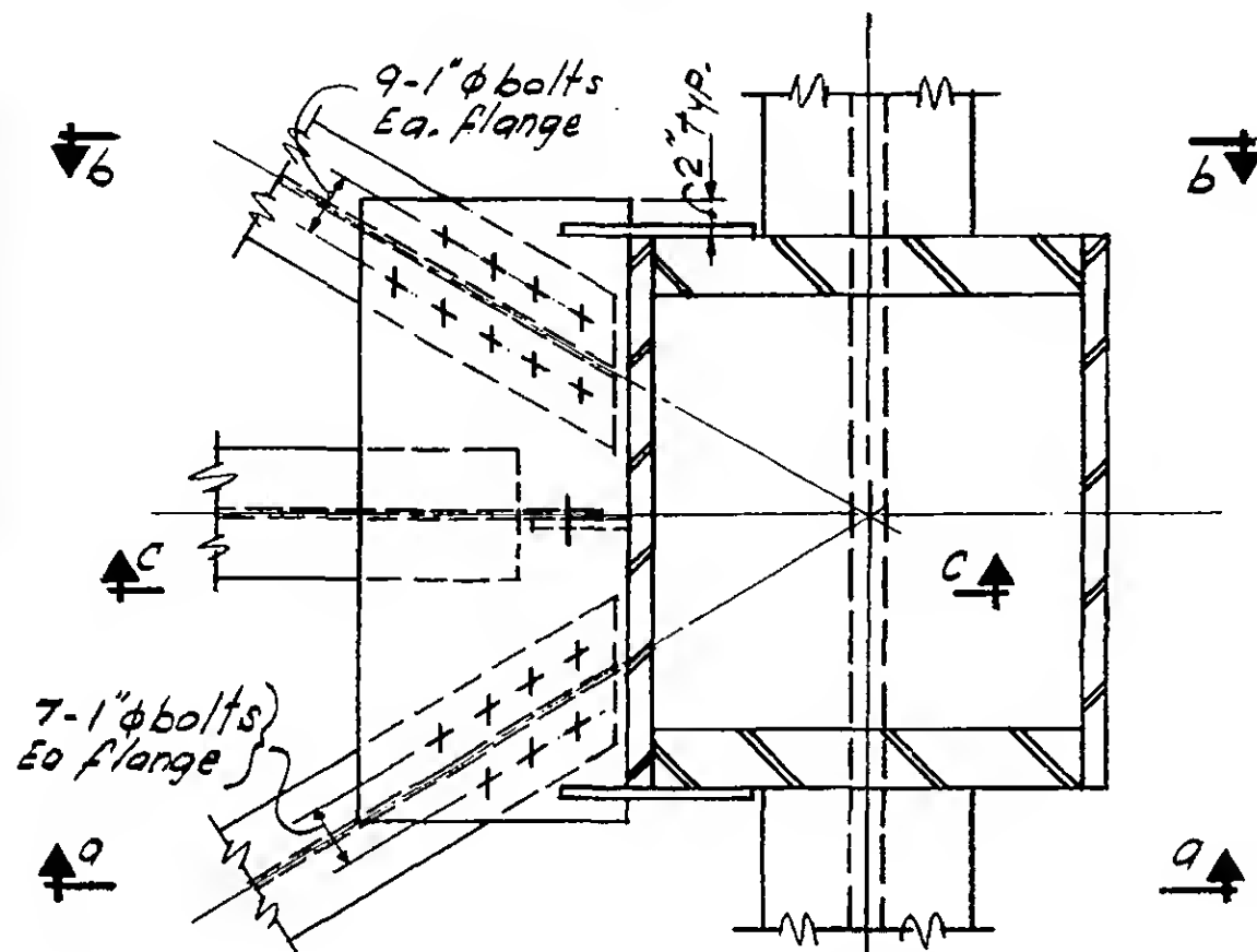
PLAN
