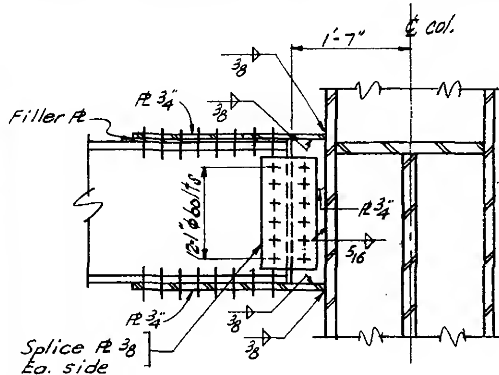
Section C-C
