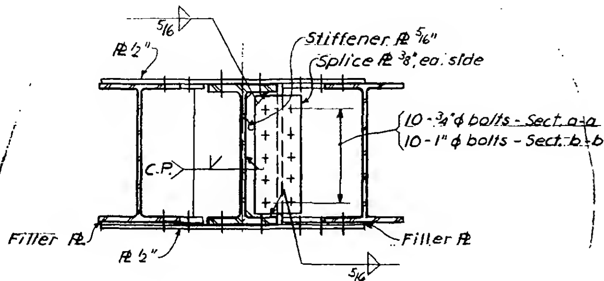
Section a-a Section b-b, opp. hand
