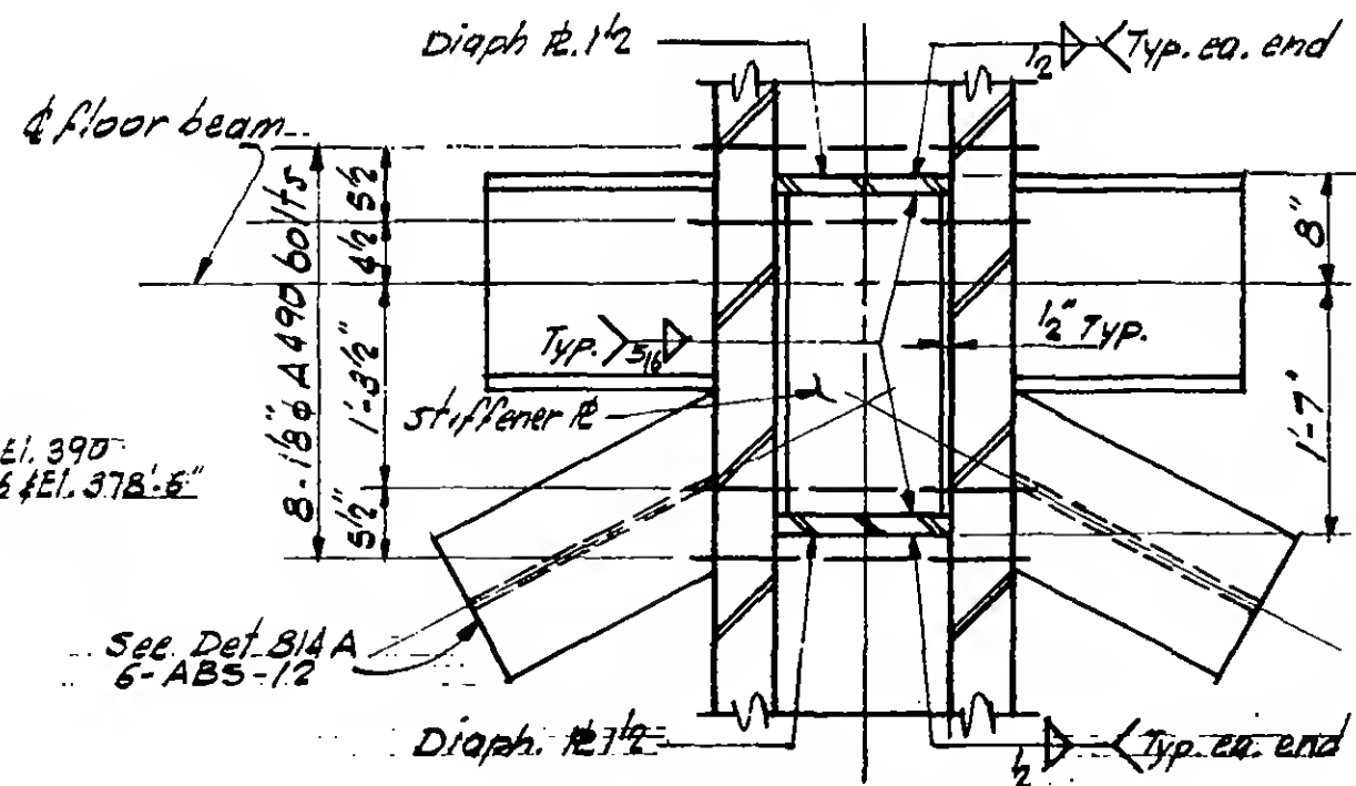
Section g-g
