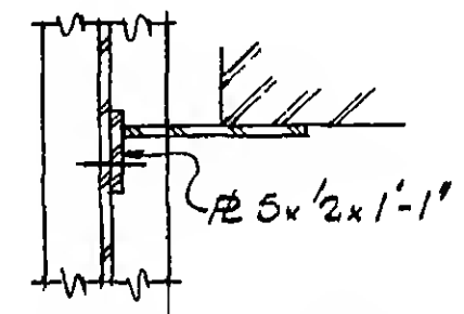
SECTION g-g
