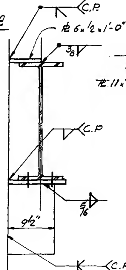
SECTION j-j
