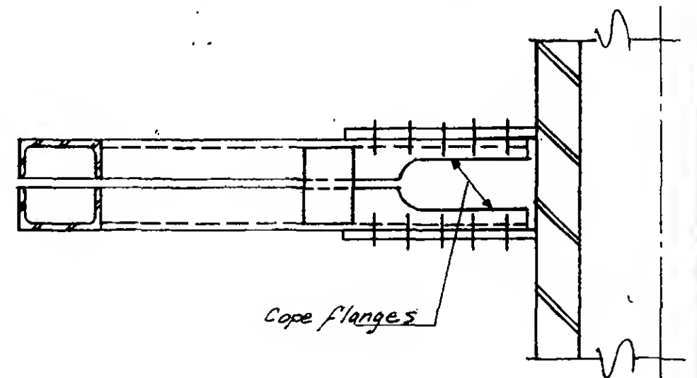
SECTION b-b
