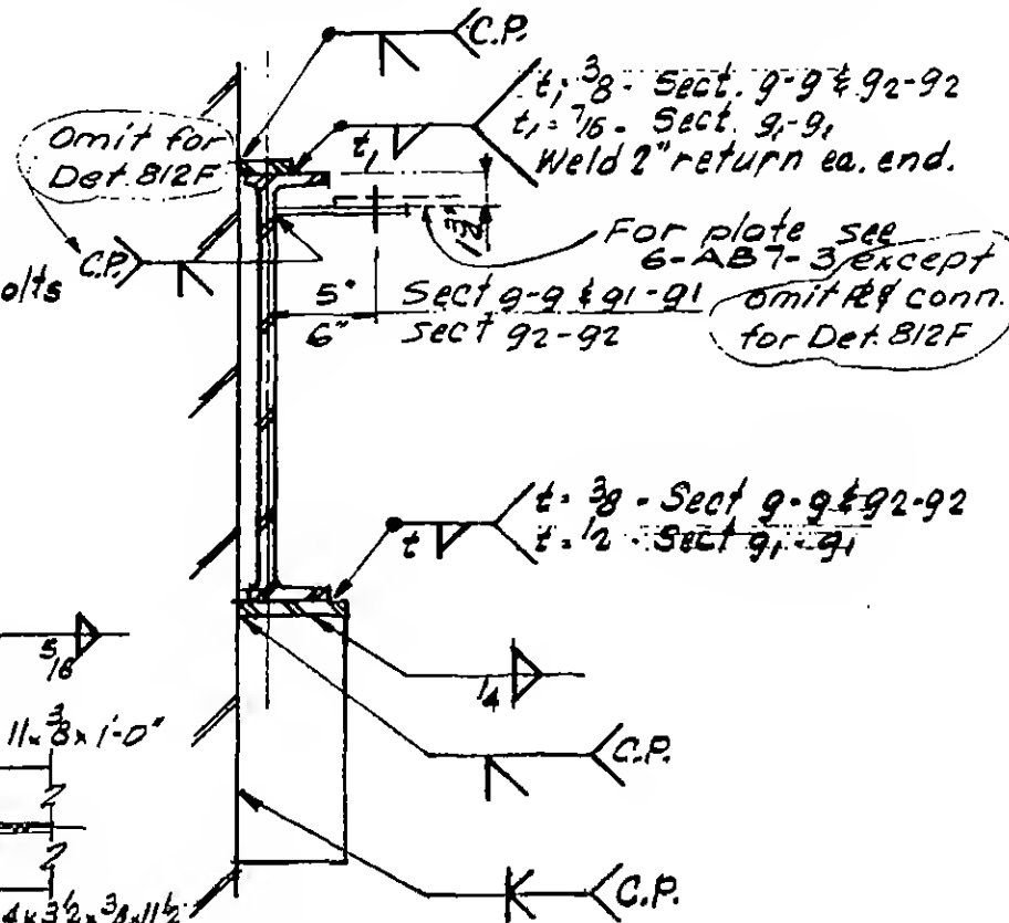
SECTION g-g, g1-g1 & g2-g2
