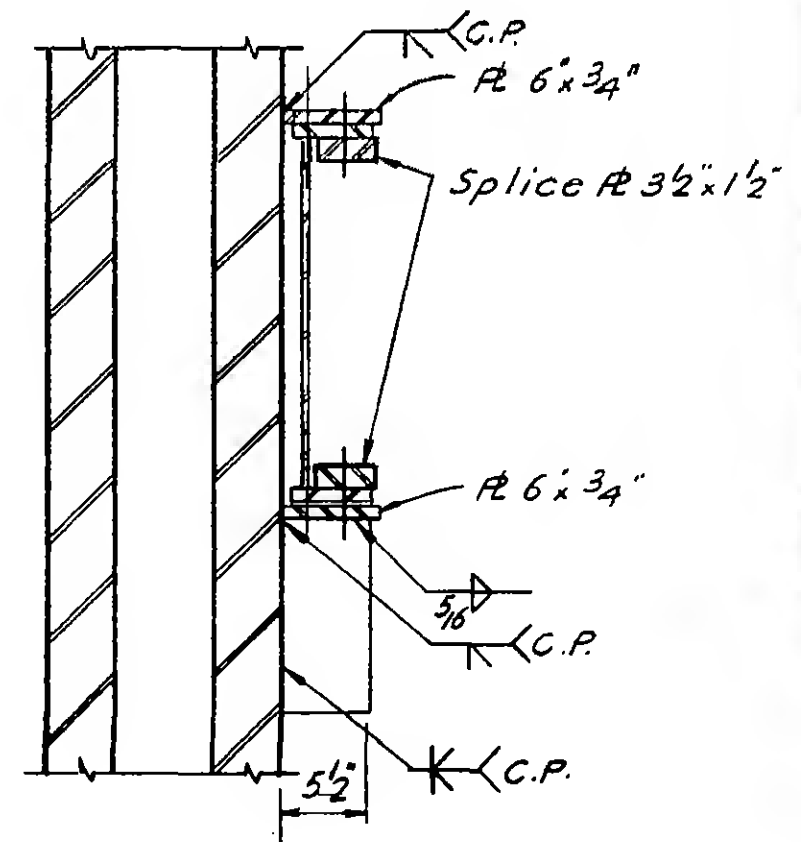
Section f-f
