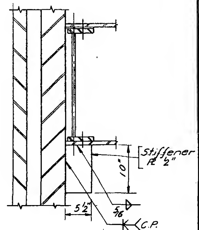
Section e-e
