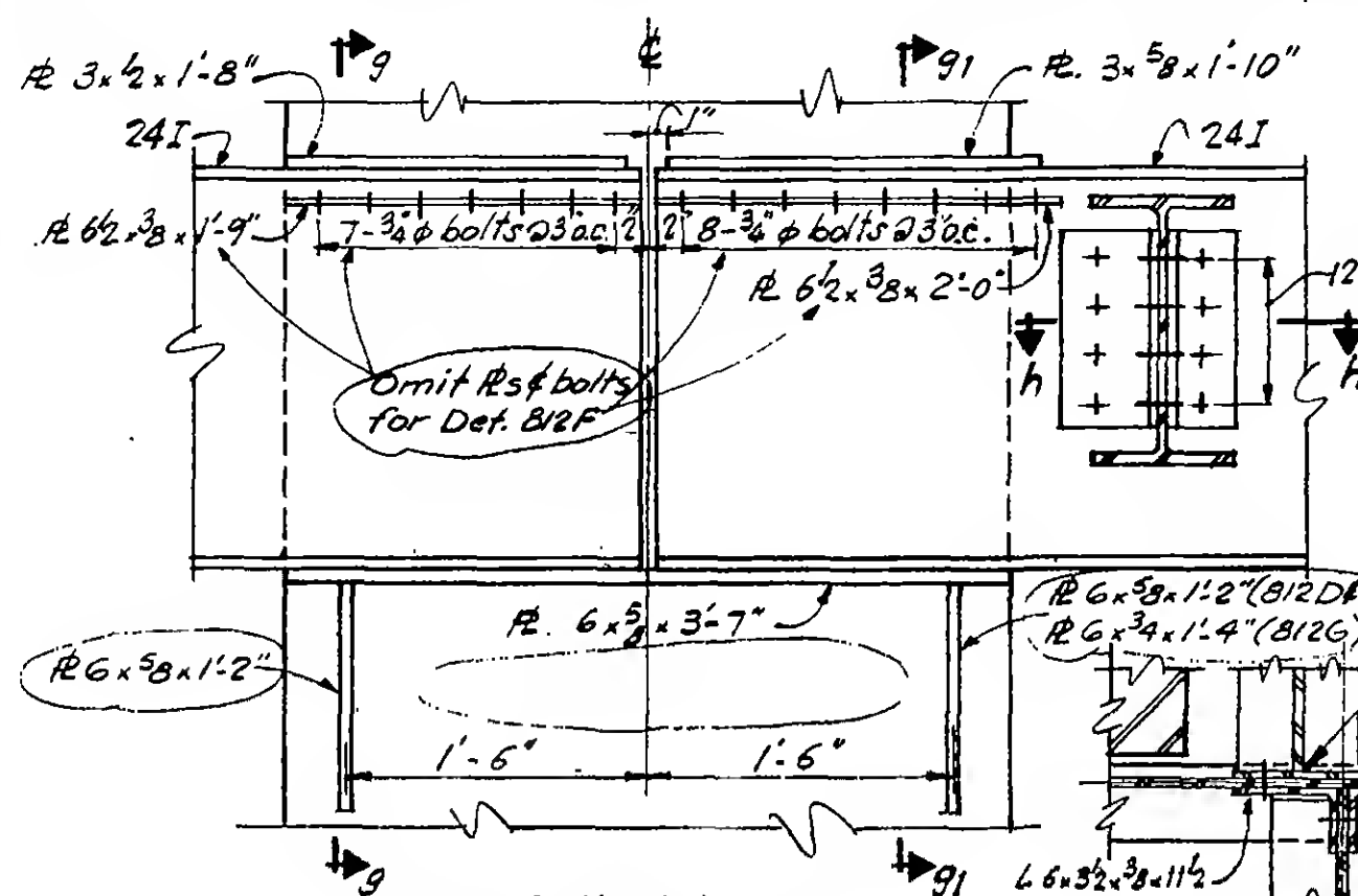
SECTION f-f
