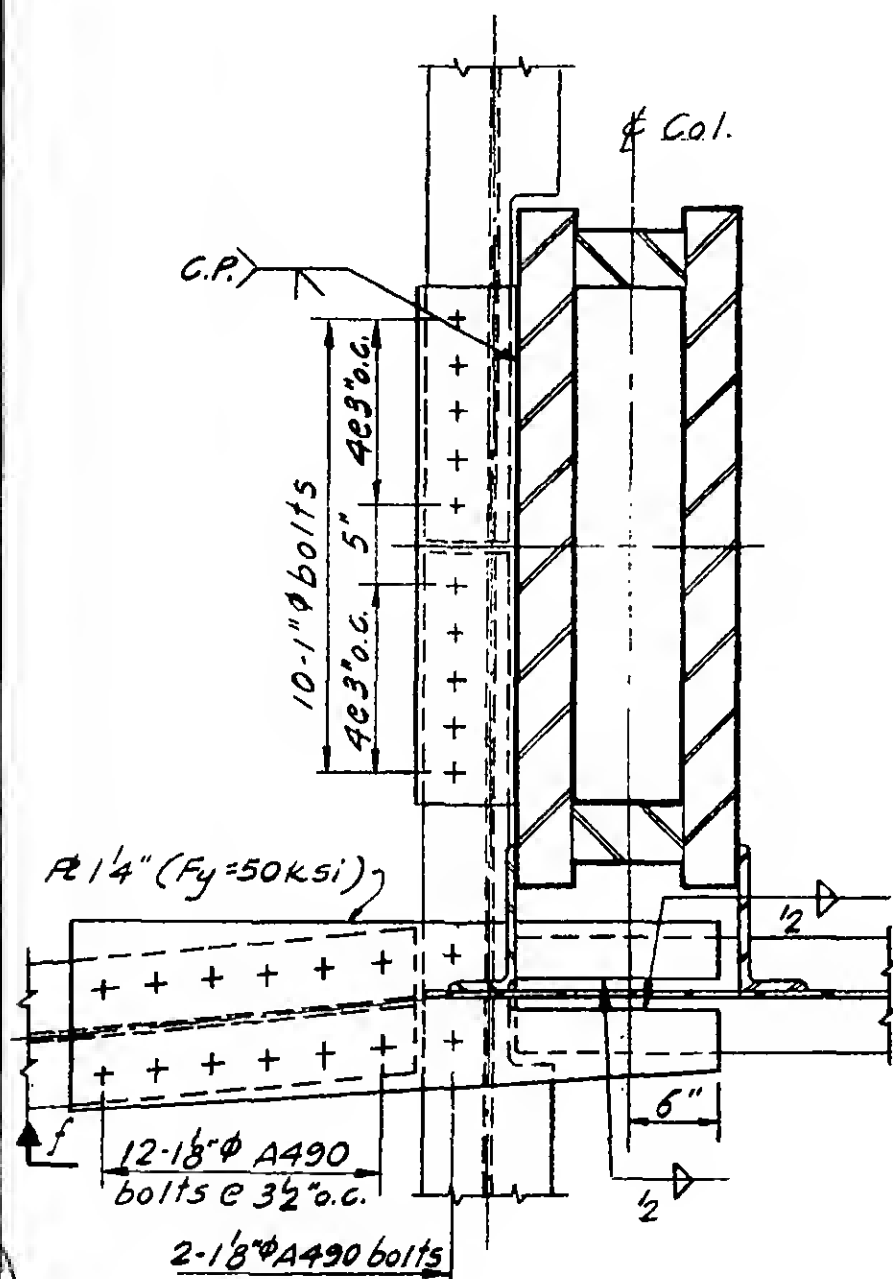
Section c-c
