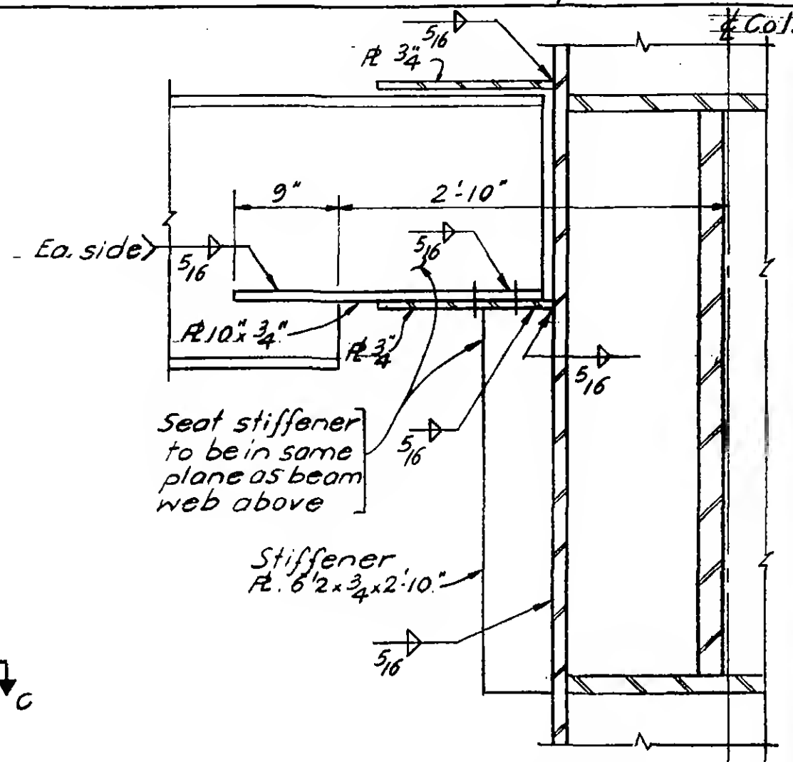
Section b-b
