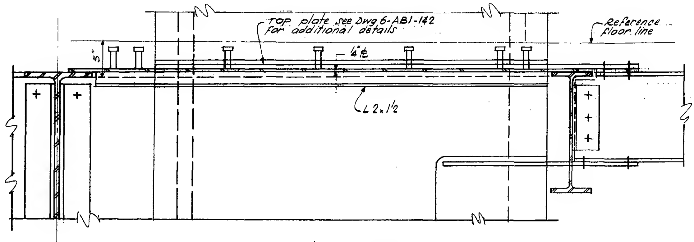
Section b-b
