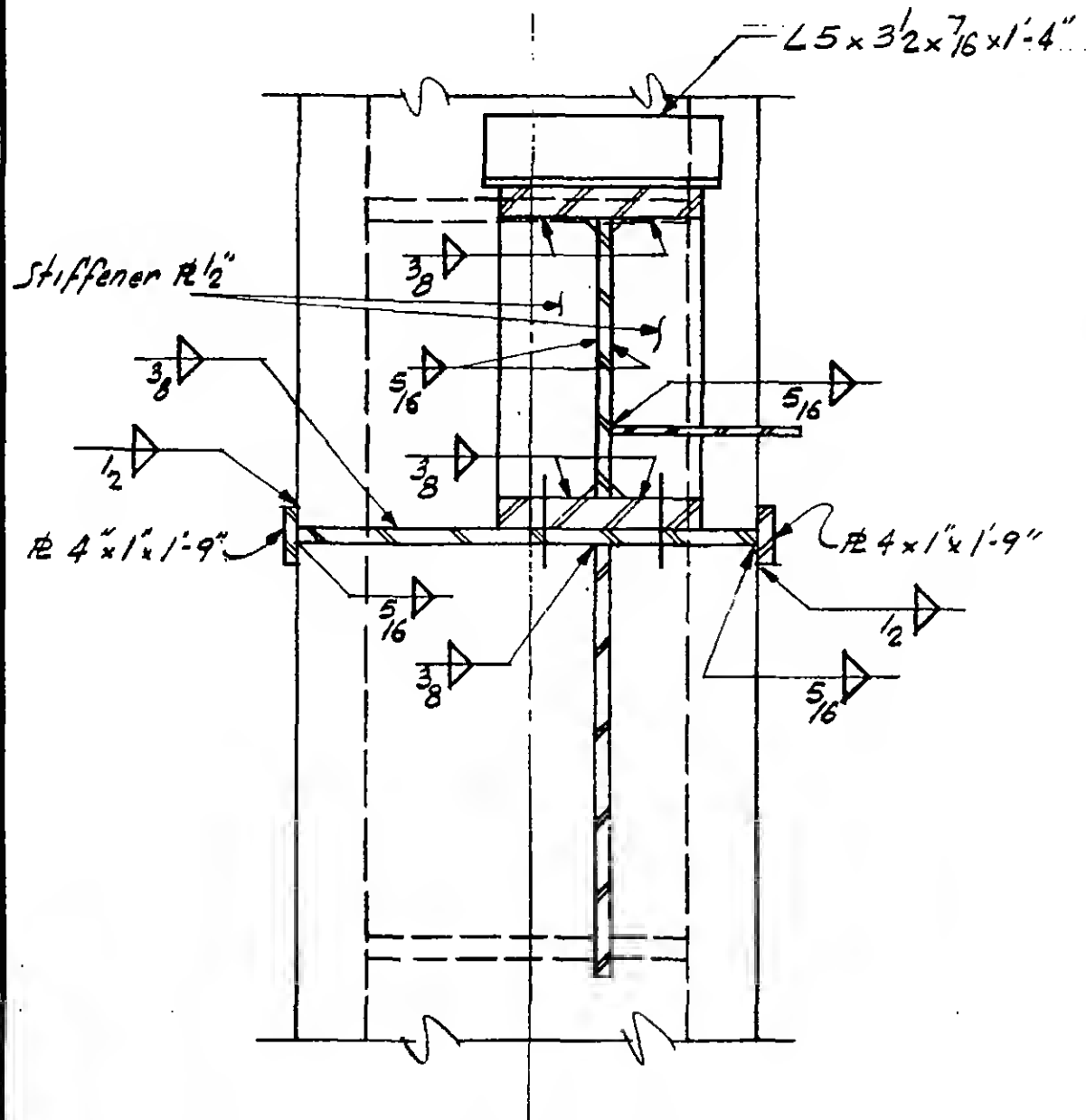
Section b-b
