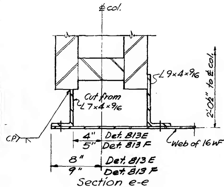
Detail 813 E & F
