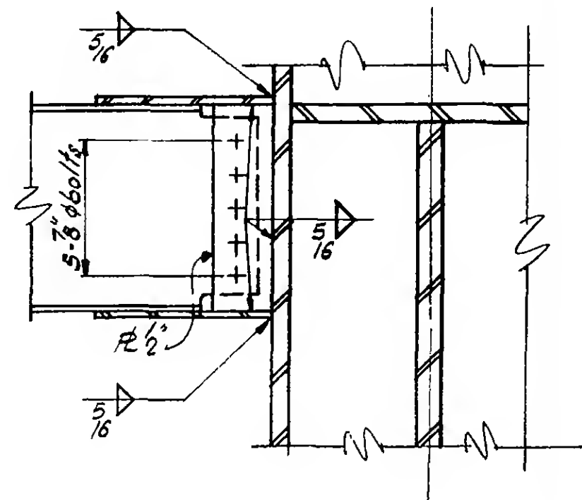
Section c-c
