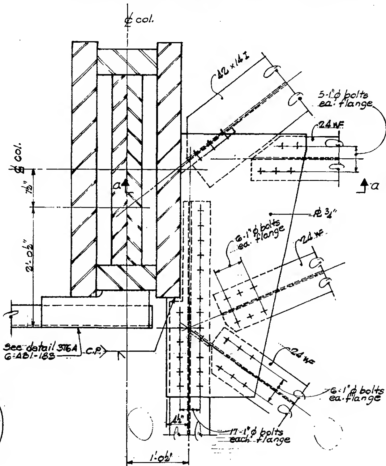
PLAN
