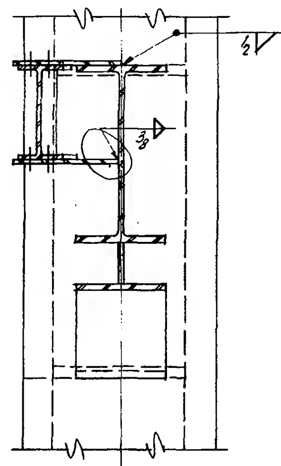
Section b-b
