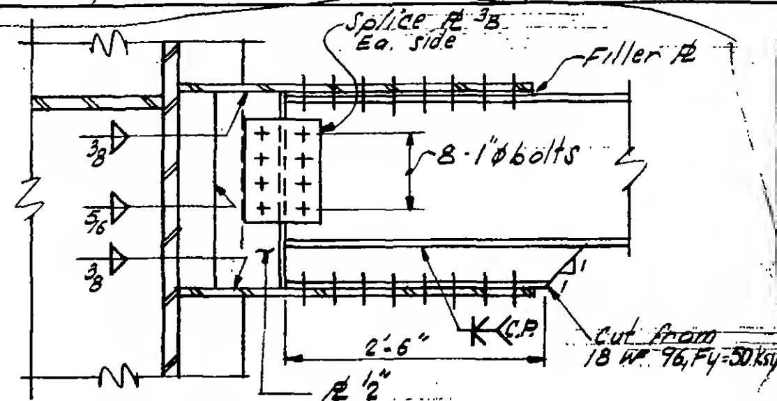
Section b-b
