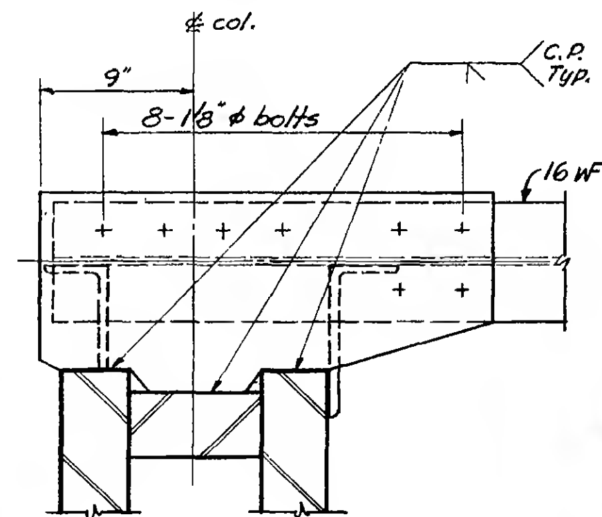
Section e-e
