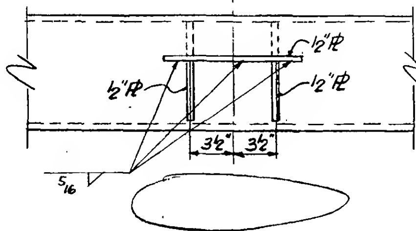
Section b-b
