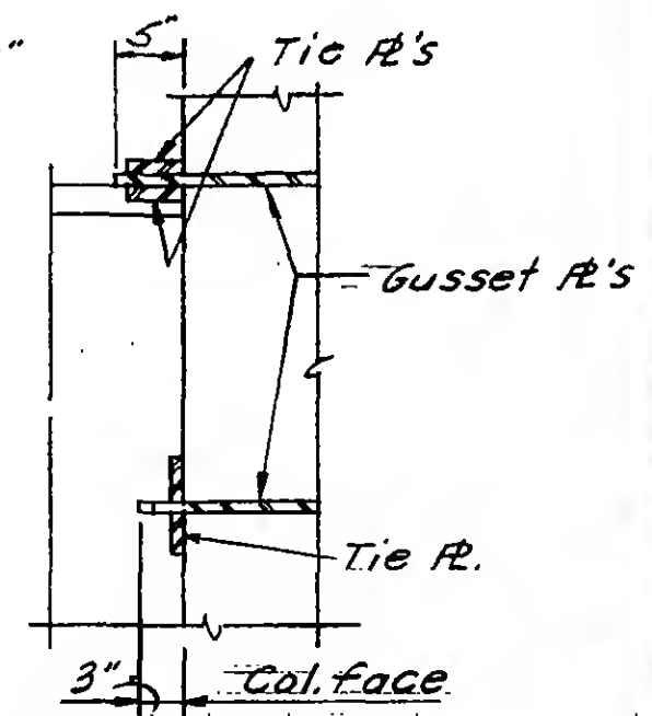
Section f-f
