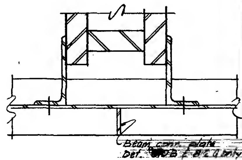
SECTION c-c
