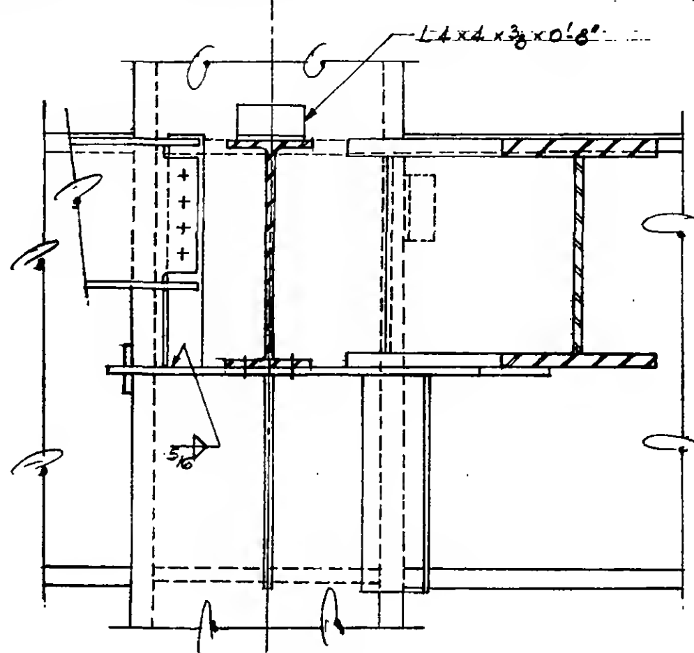
Section e-e
