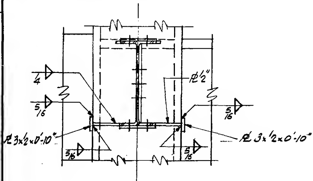
Section b-b
