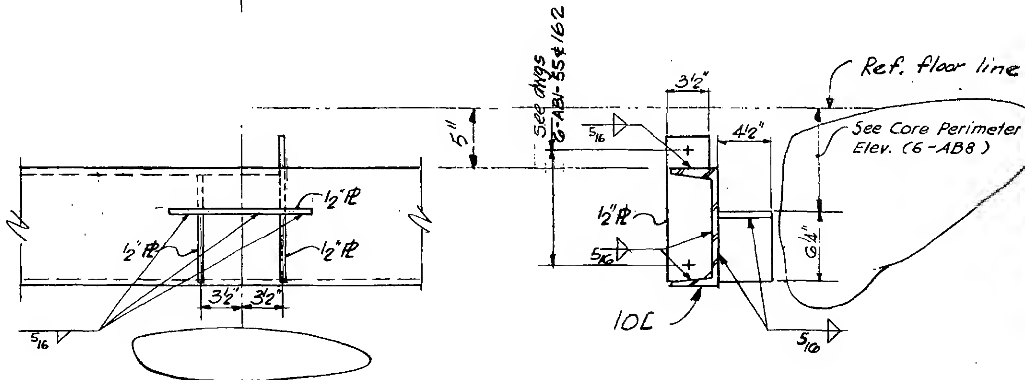
Section c-c
