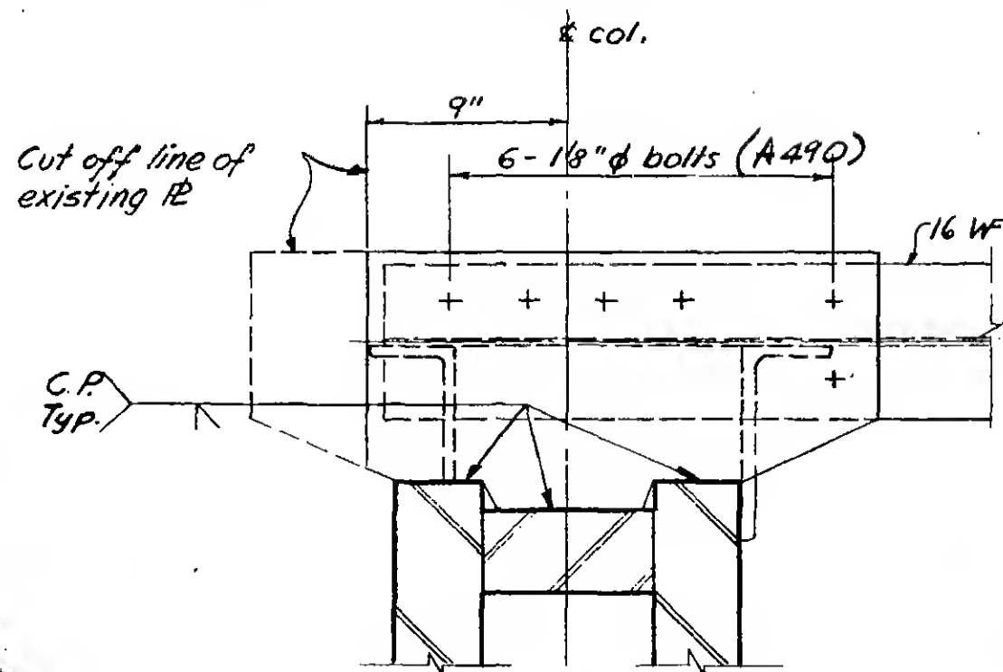
Section e-e
