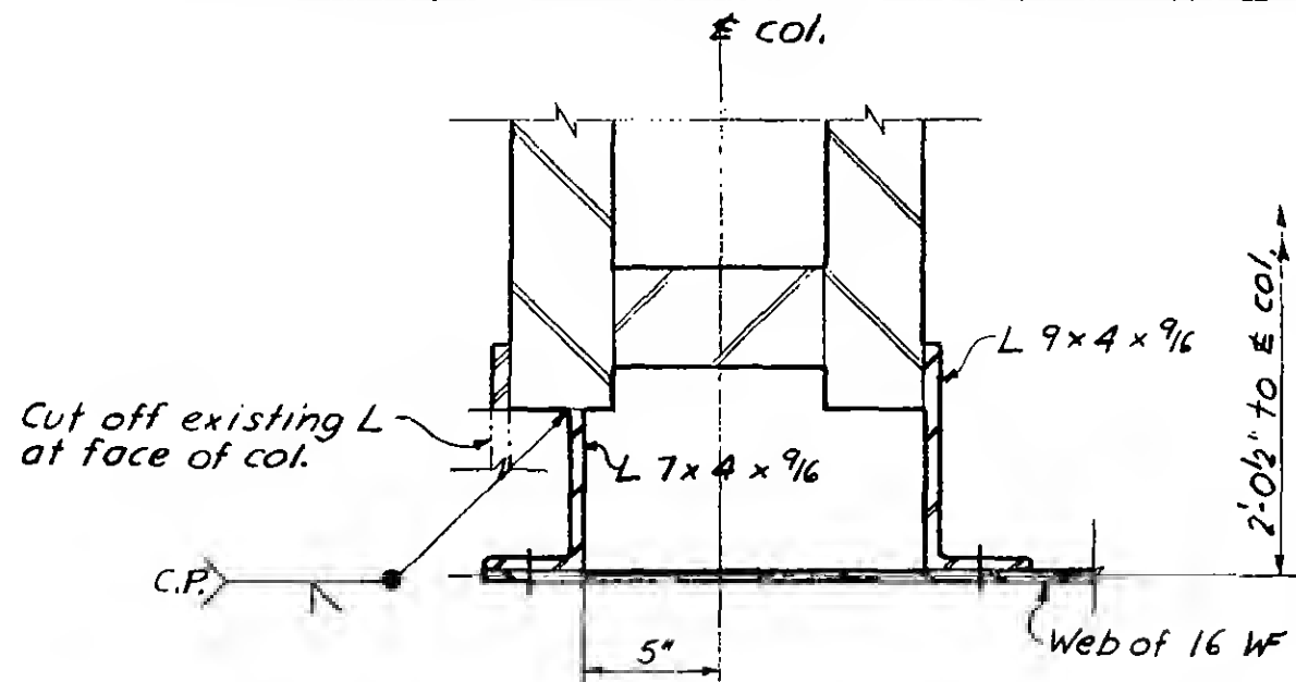
Section e-e
