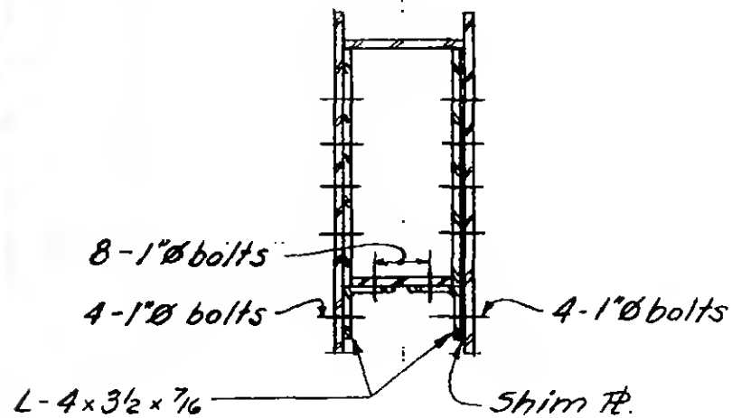
Section c-c
