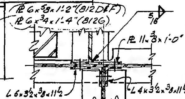
SECTION h-h
