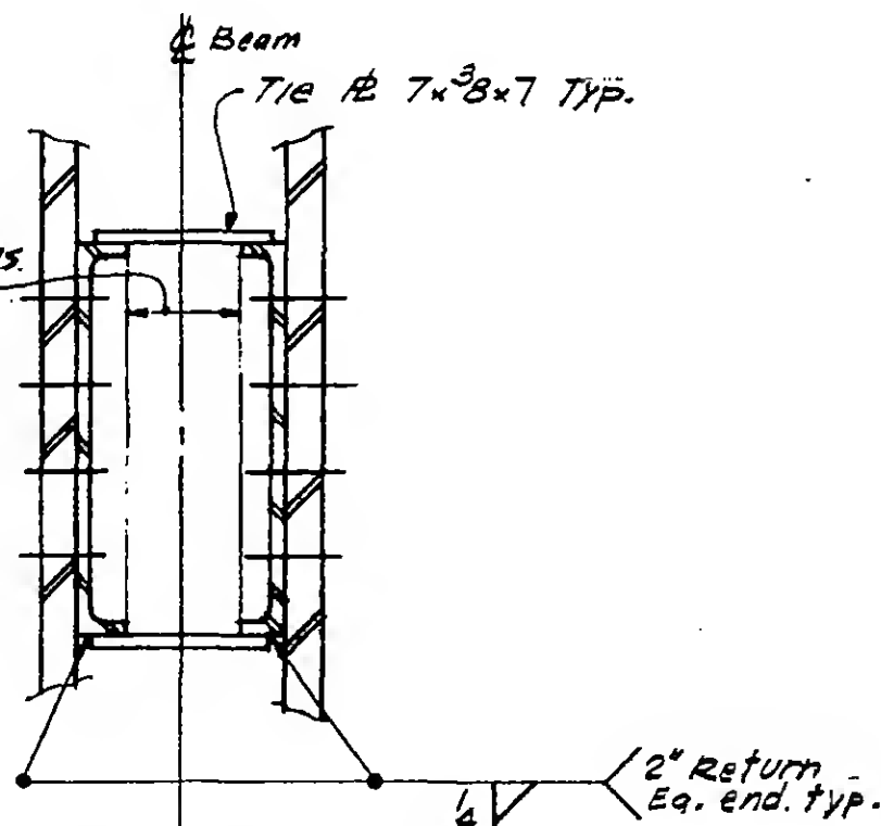
SECTION b-b
