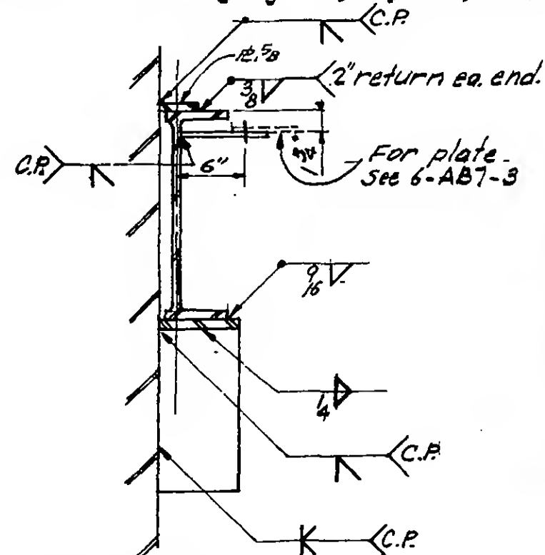
SECTION k-k
