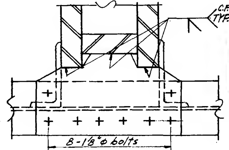
SECTION b-b (SECTION d-d Similar)
