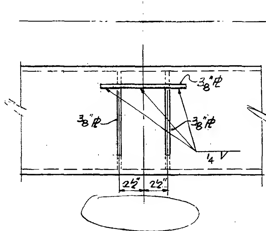
Section b-b
