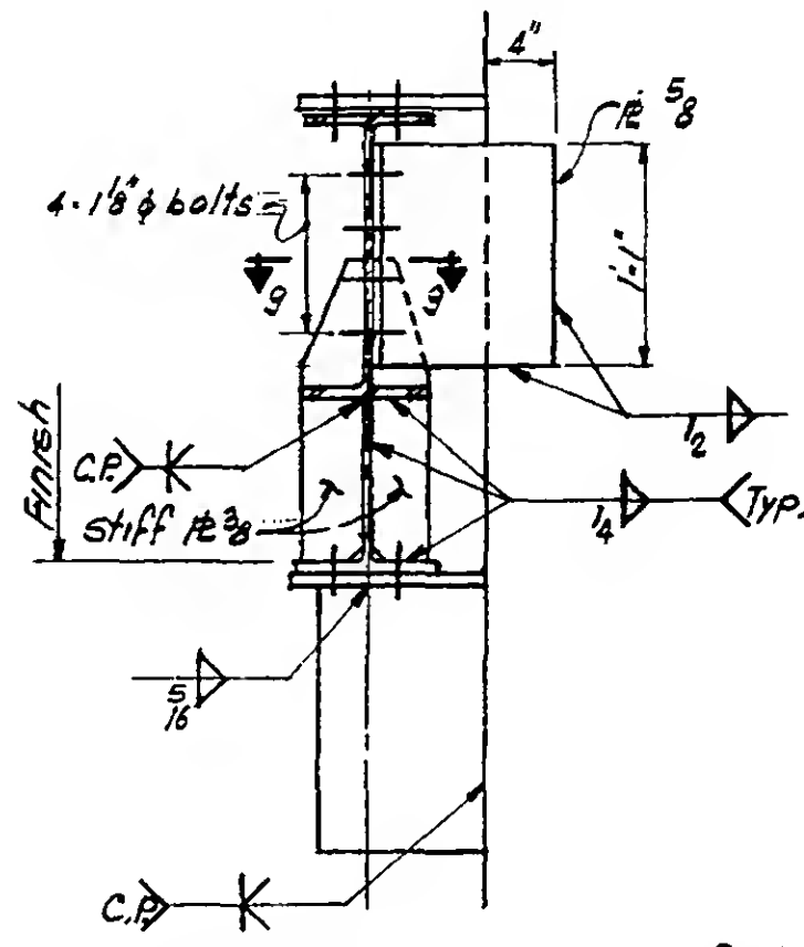
SECTION e-e
