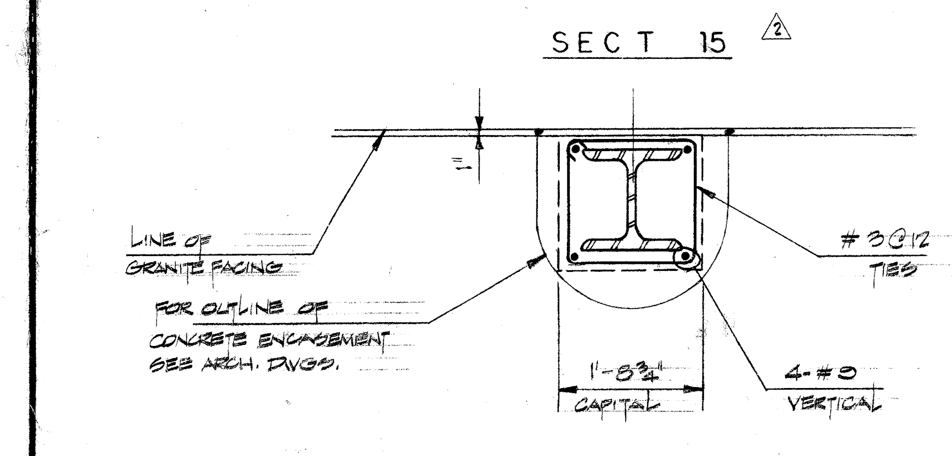
TYPICAL DETAIL OF COLUMN ENCASEMENT WITHOUT DRAINS
