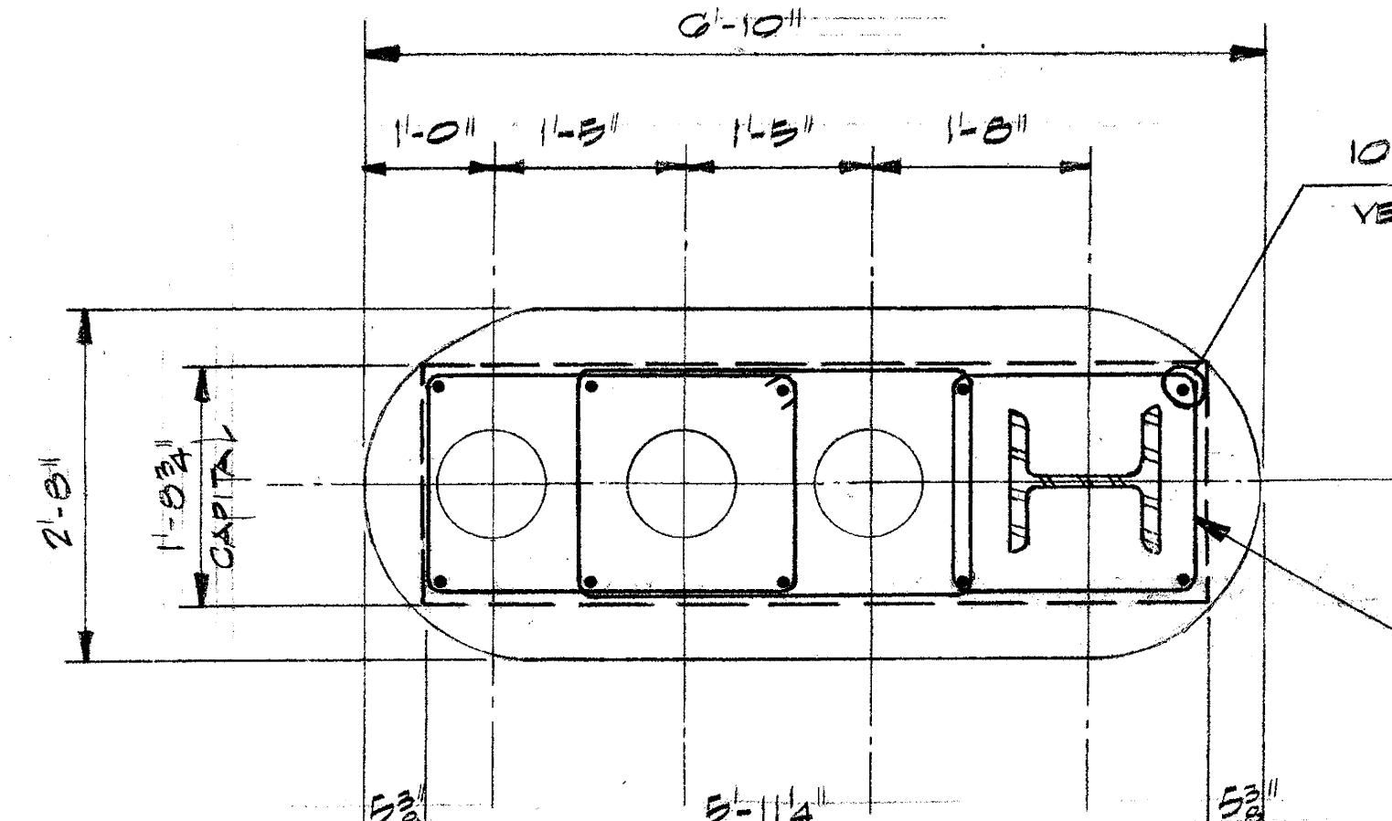
TYPICAL DETAIL OF COLUMN ENCASEMENT WITH DRAINS
