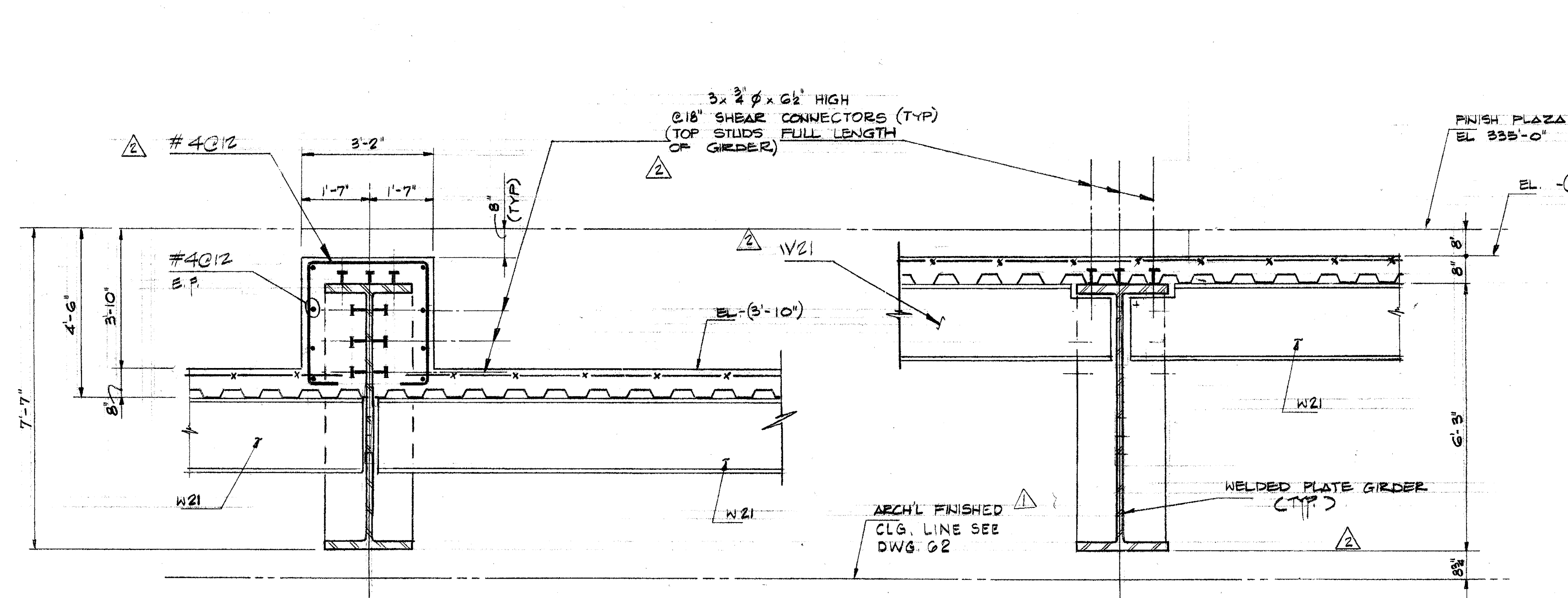
TYPICAL SECTION
