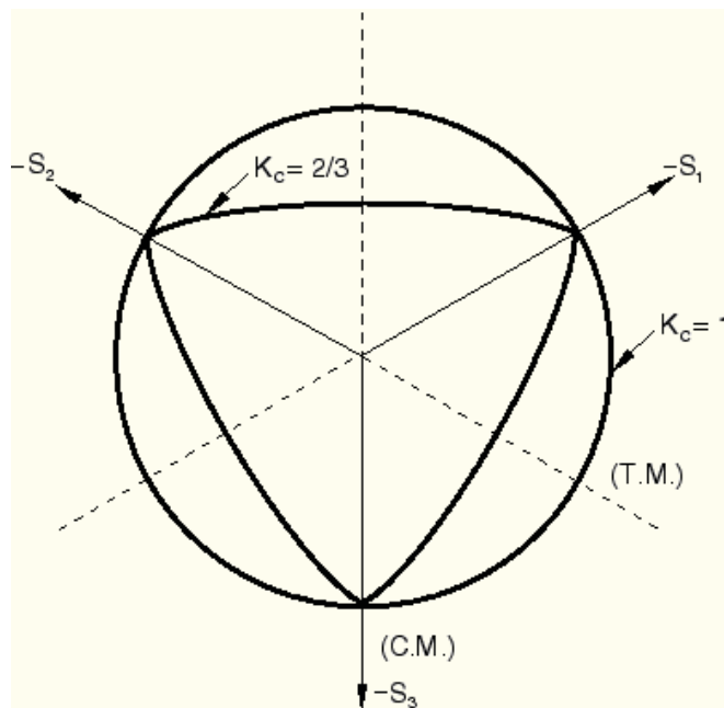
Figure 146: Damaged Plasticity model Yield Surface in Deviatoric Plane
