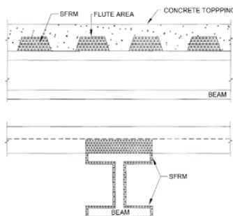
Figure 8 Flutes filled with SFRM when deck is perpendicular to beams 10
