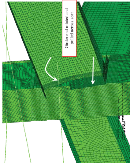
Figure 17: 700°C Unfillet Flutes Case 1 - Column 79 Seated Connection at End of Cooling
