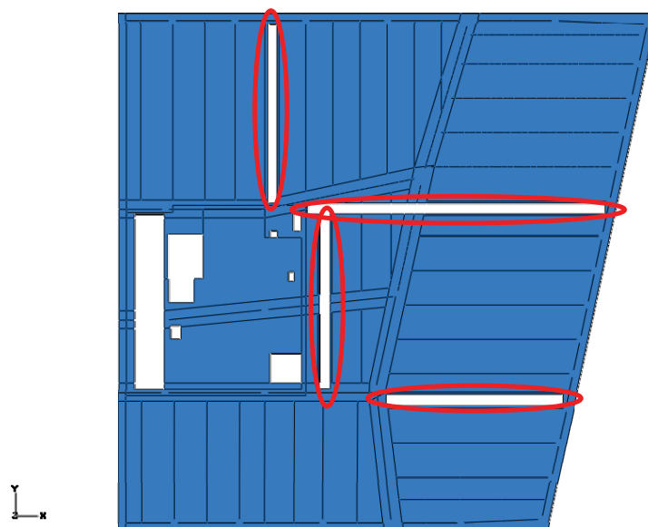
Figure 136: Trench headers locations in the ABAQUS sub-model (circled in red)
