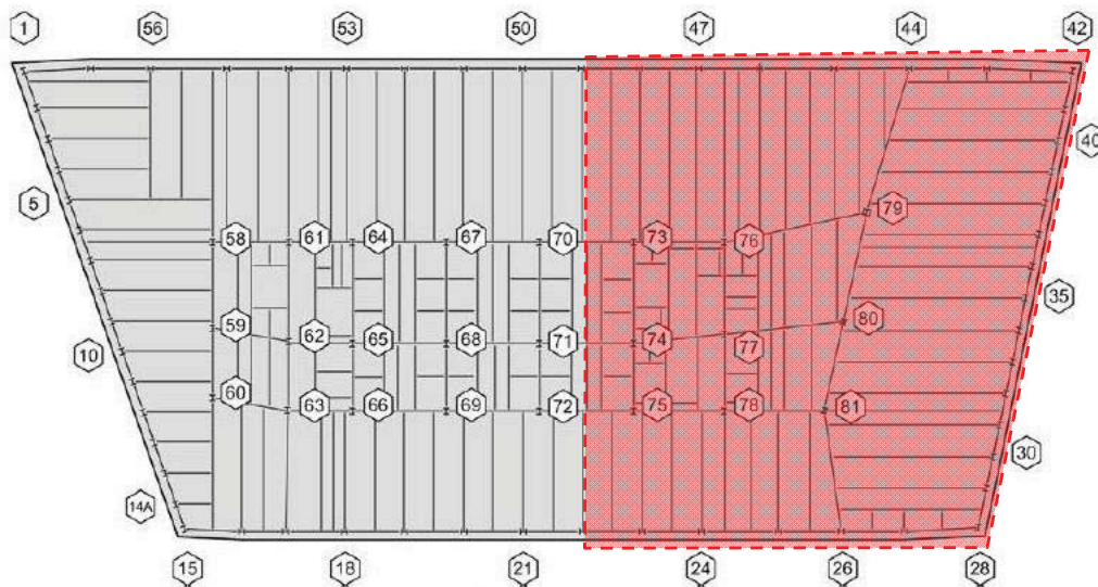
Figure 133: Extent of proposed detailed model (shaded in red) of level 13
